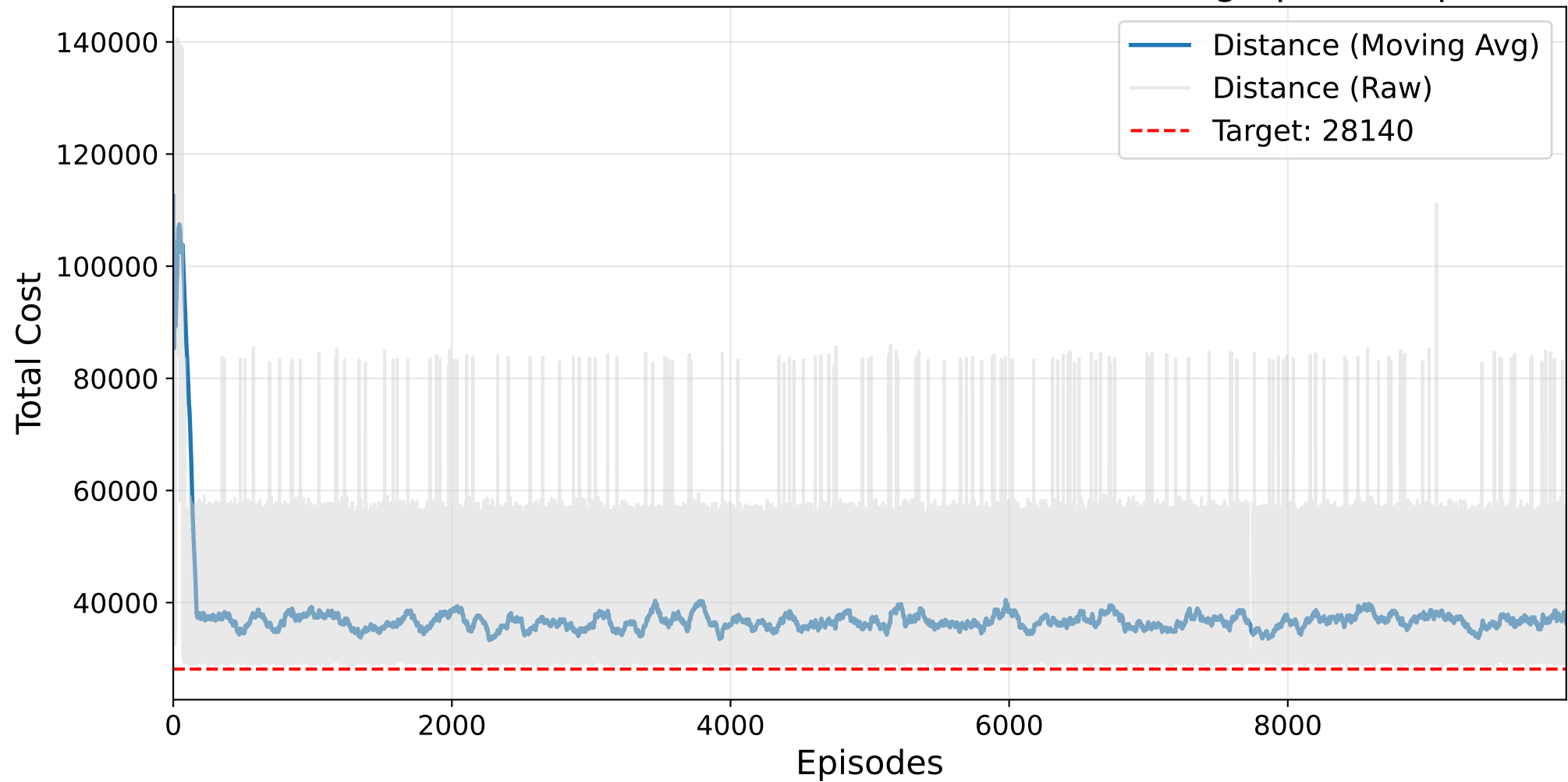
Final HYPERBAND TPE Masked AutoRL-SOP Training - p43.1.sop
